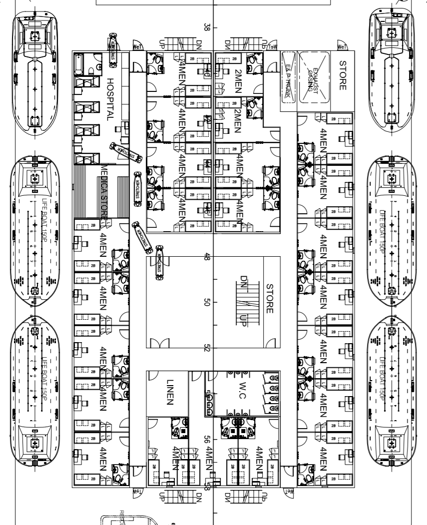
ACCOMMODATION DECK 2 22 X 4 MEN = 88 MEN 2 X 2 MEN = 4 MEN TOTAL = 92 MEN
