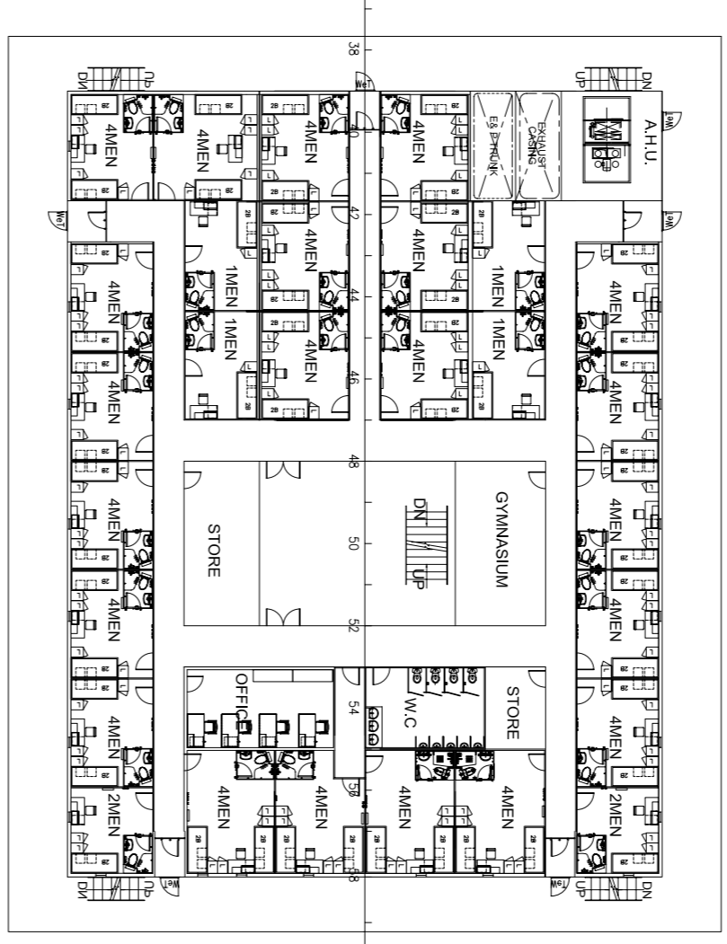
ACCOMMODATION DECK 4 22 X 4 MEN = 88 MEN 2 X 2 MEN = 4 MEN 4 X 1 MEN = 4 MEN TOTAL = 98 MEN
