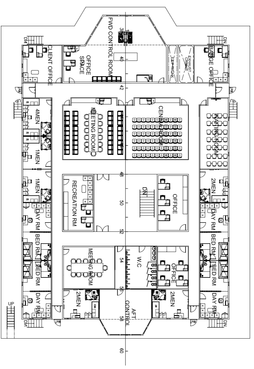
ACCOMMODATION DECK 6 1 X 4 MEN = 4 MEN 5 X 1 MEN = 5 MEN 6 X 1 MEN = 6 MEN TOTAL = 16 MEN
