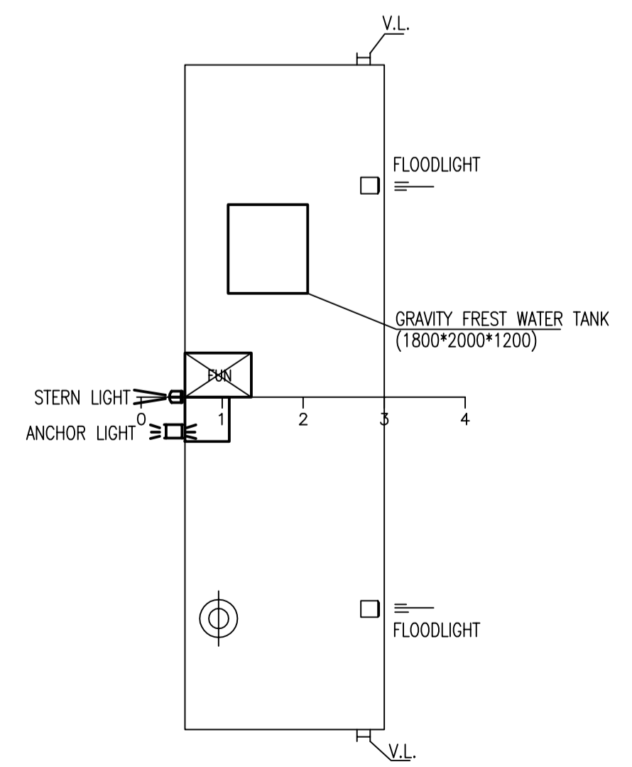
DECK HOUSE TOP
