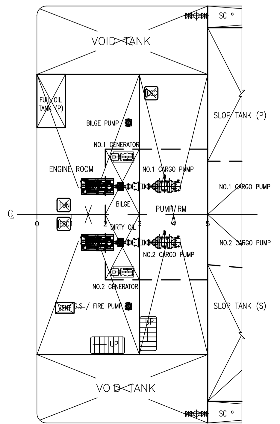
ENGINE/PUMP ROOM PLAN
