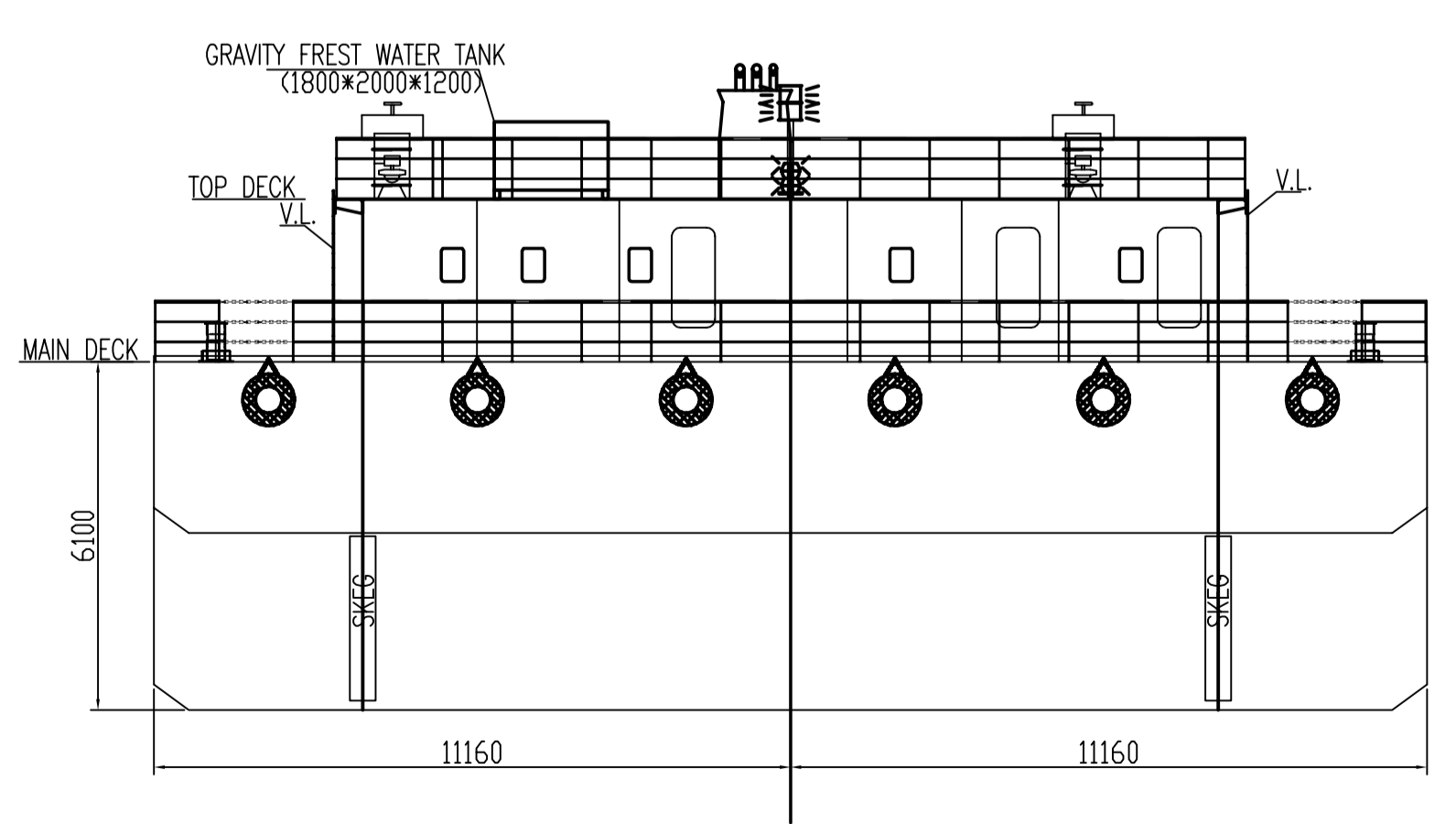
AFTER VIEW
