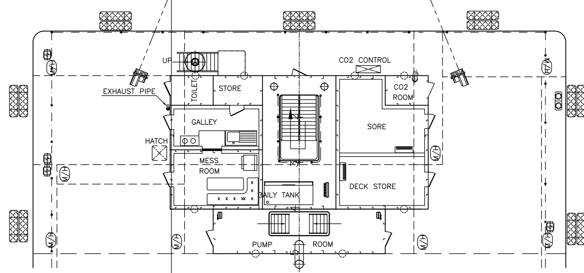
MAIN DECK 1:100
