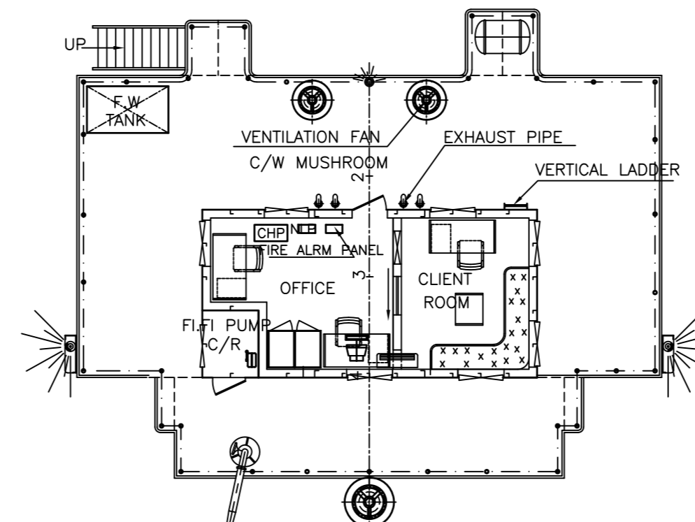
FIRST DECK 1:100
