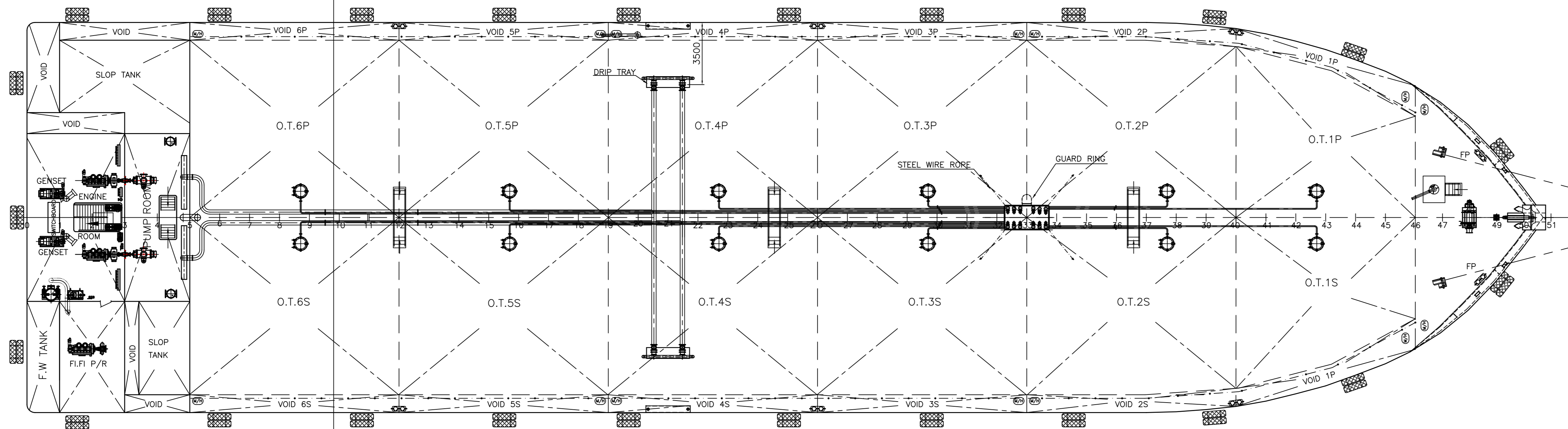
MAIN DECK
