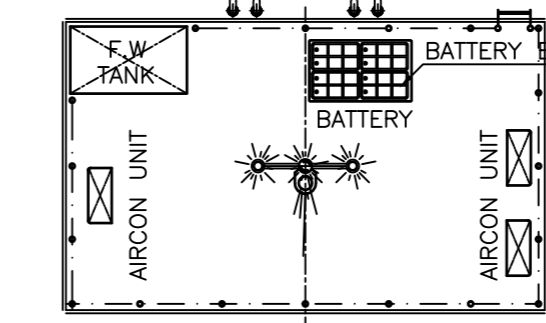
DECK HOUSE TOP 1:100
