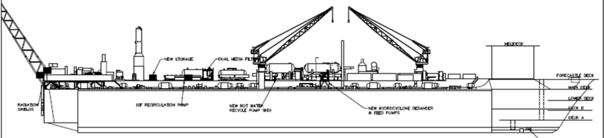
ELEVATION - MING ZHU FPSO
