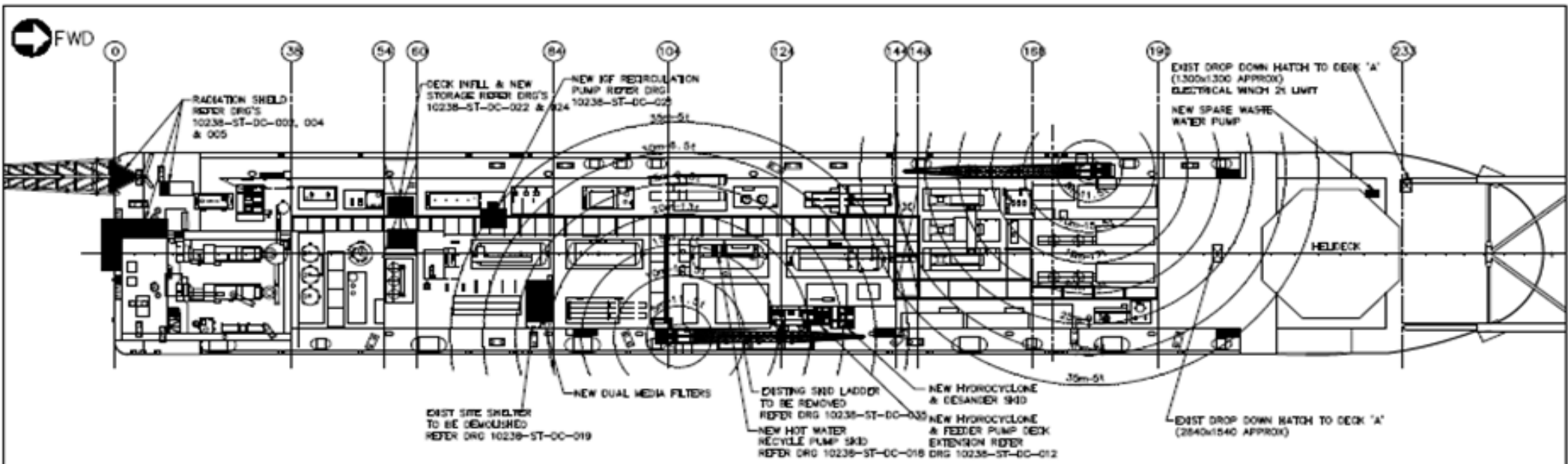
PLAN - MING ZHU FPSO
