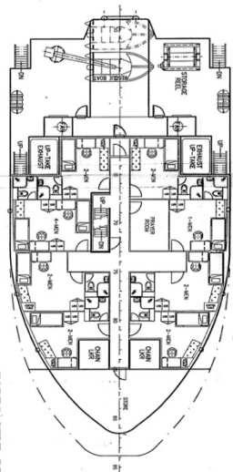
FORECASTLE DECK
